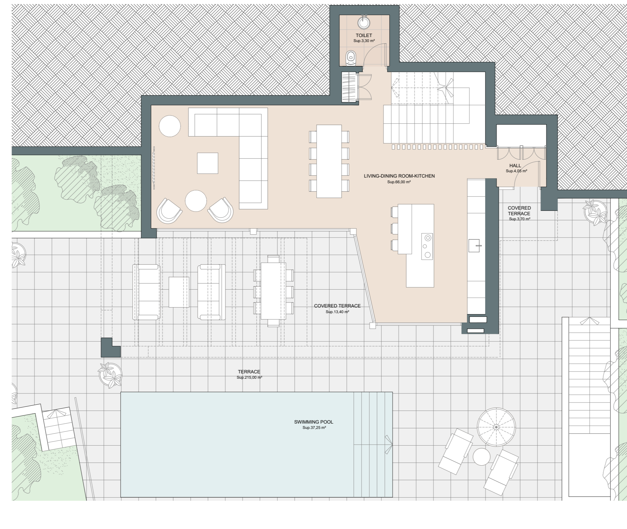
GROUND FLOOR
